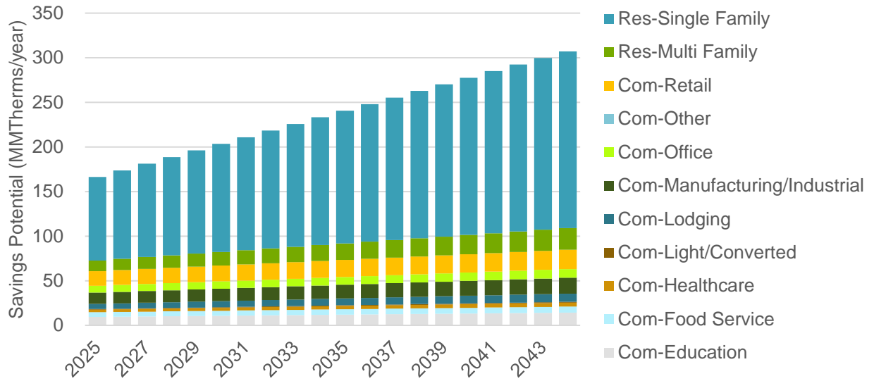
Figure C-1. Natural Gas Technical Potential by Customer Segment (MMTherms/year)
