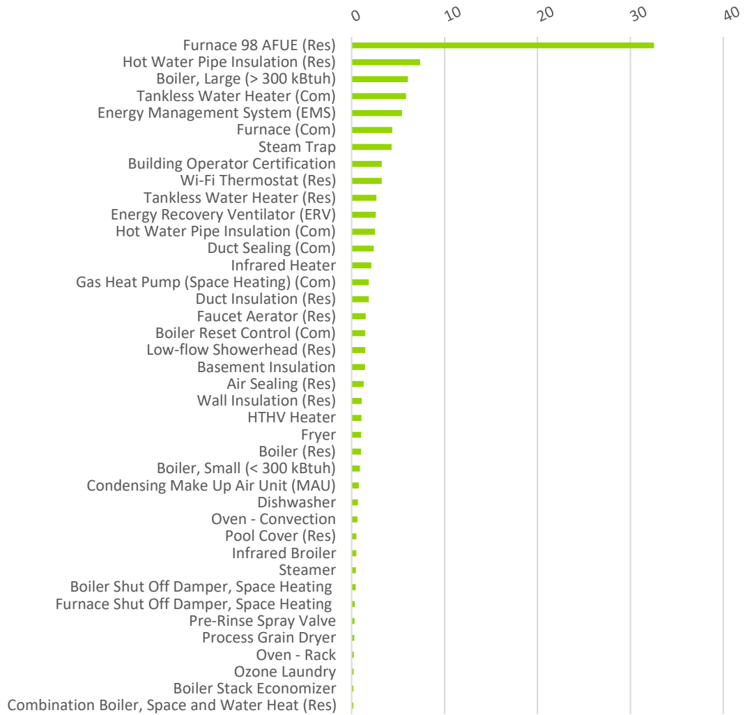
Figure D-2. Top 40 Measures - Natural Gas Economic Potential in 2024 (MMTherms/year)
