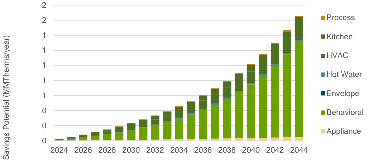
Figure E-12. Cumulative Net Natural Gas Achievable Potential by Commercial Sector End Use (MMTherms/year)
