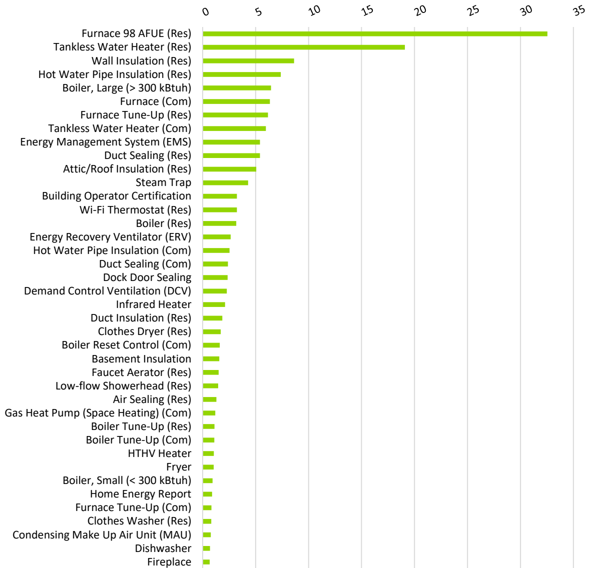
Figure C-2. Top 40 Measures - Natural Gas Technical Potential in 2024 (MMTherms/year)
