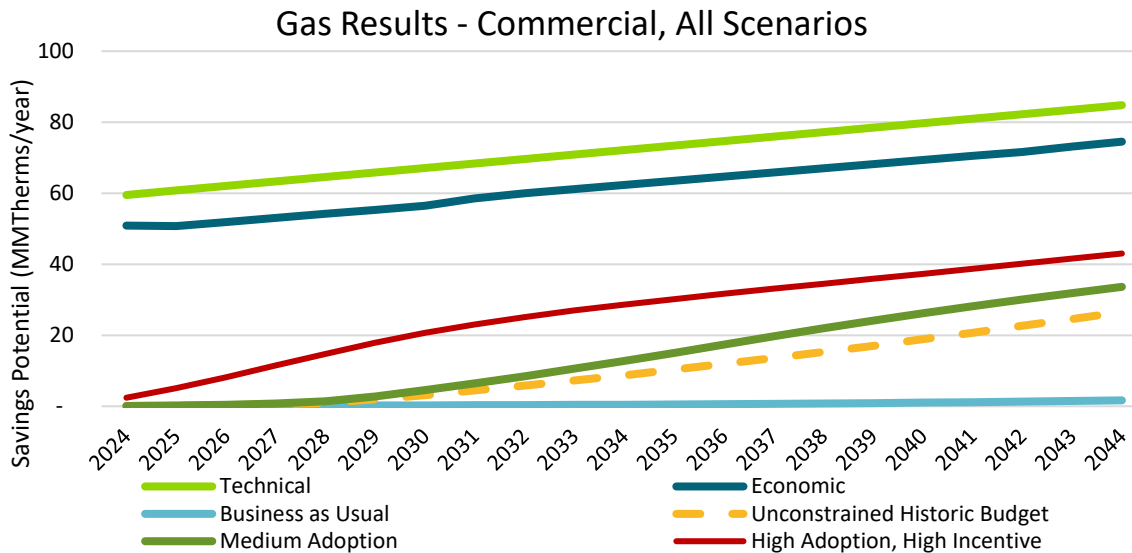
Figure E-17. Commercial Natural Gas Cumulative Energy Results by Scenario (MMTherms/year)
