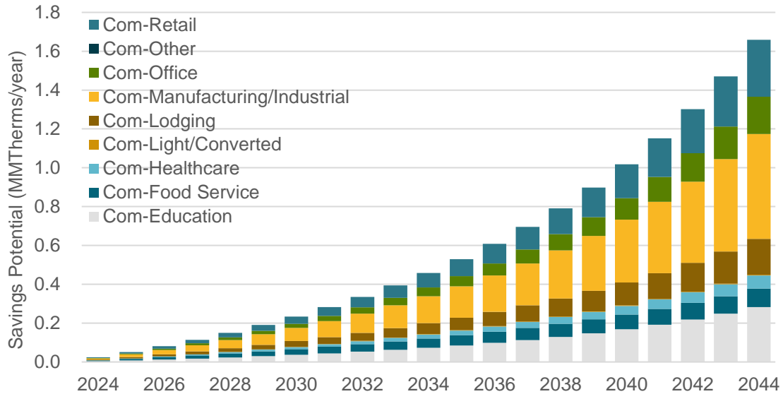
Figure E-10. Cumulative Net Natural Gas Achievable Potential by Commercial Customer Segment (MMTherms/year)
