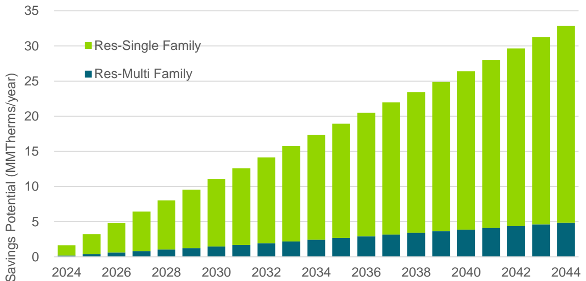
Figure E-9. Cumulative Net Natural Gas Achievable Potential by Residential Customer Segment (MMTherms/year)
