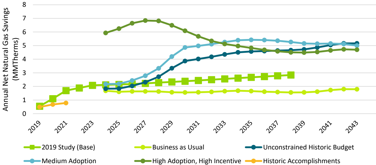
Figure 5-6. Natural Gas Historic Accomplishments Compared to Past and Current Study All Achievable Potential Scenario Results (Annual Net Gas Savings MMTherms)
